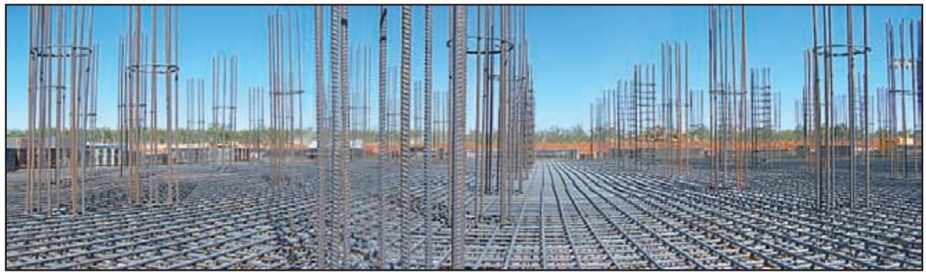
MORANBAH - DYNO NOBEL - AMMONIUM TANK FOUNDATION 400m 3 CONCRETE / 50 TONNES OF STEEL POUR COMMENCED MIDNIGHT AND TOOK 8 HOURS TO PLACE CONCRETE
