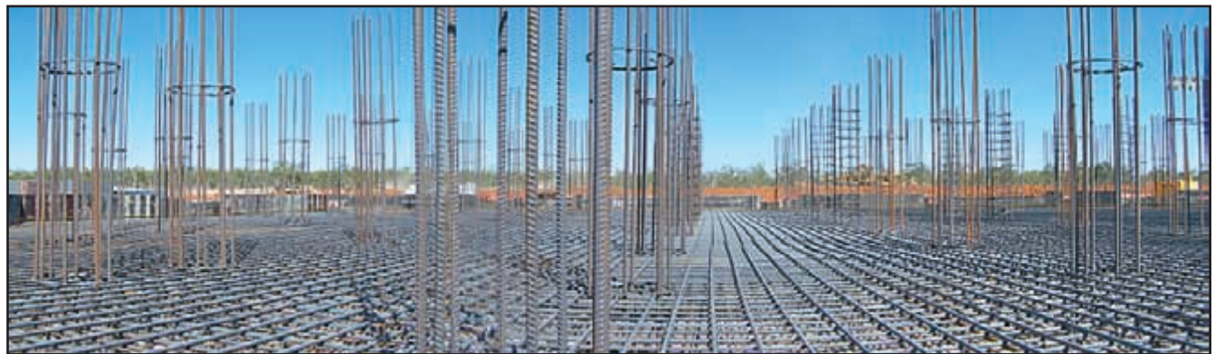
MORANBAH - DYNO NOBEL - AMMONIUM TANK FOUNDATION 400m 3 CONCRETE / 50 TONNES OF STEEL POUR COMMENCED MIDNIGHT AND TOOK 8 HOURS TO PLACE CONCRETE
